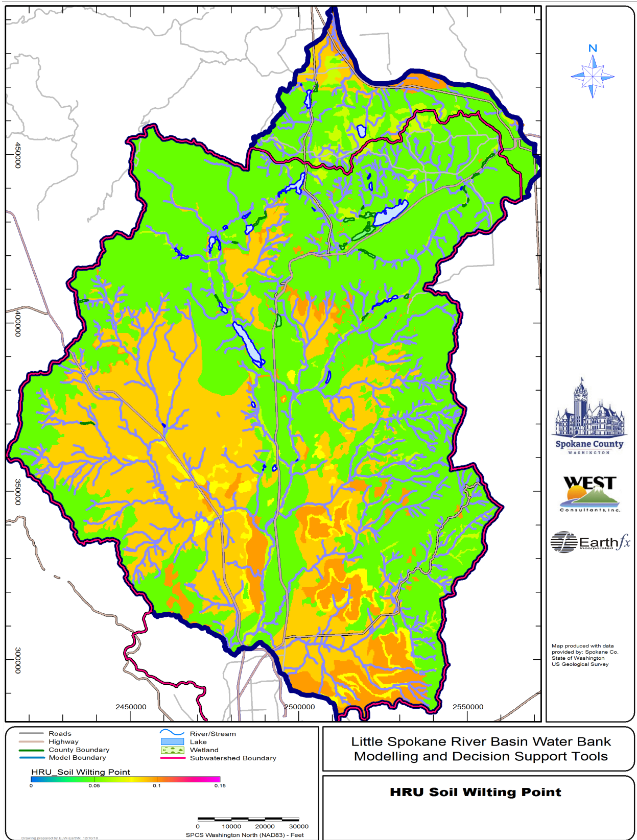
Figure 7.21: Distribution of soil zone wilting point.
