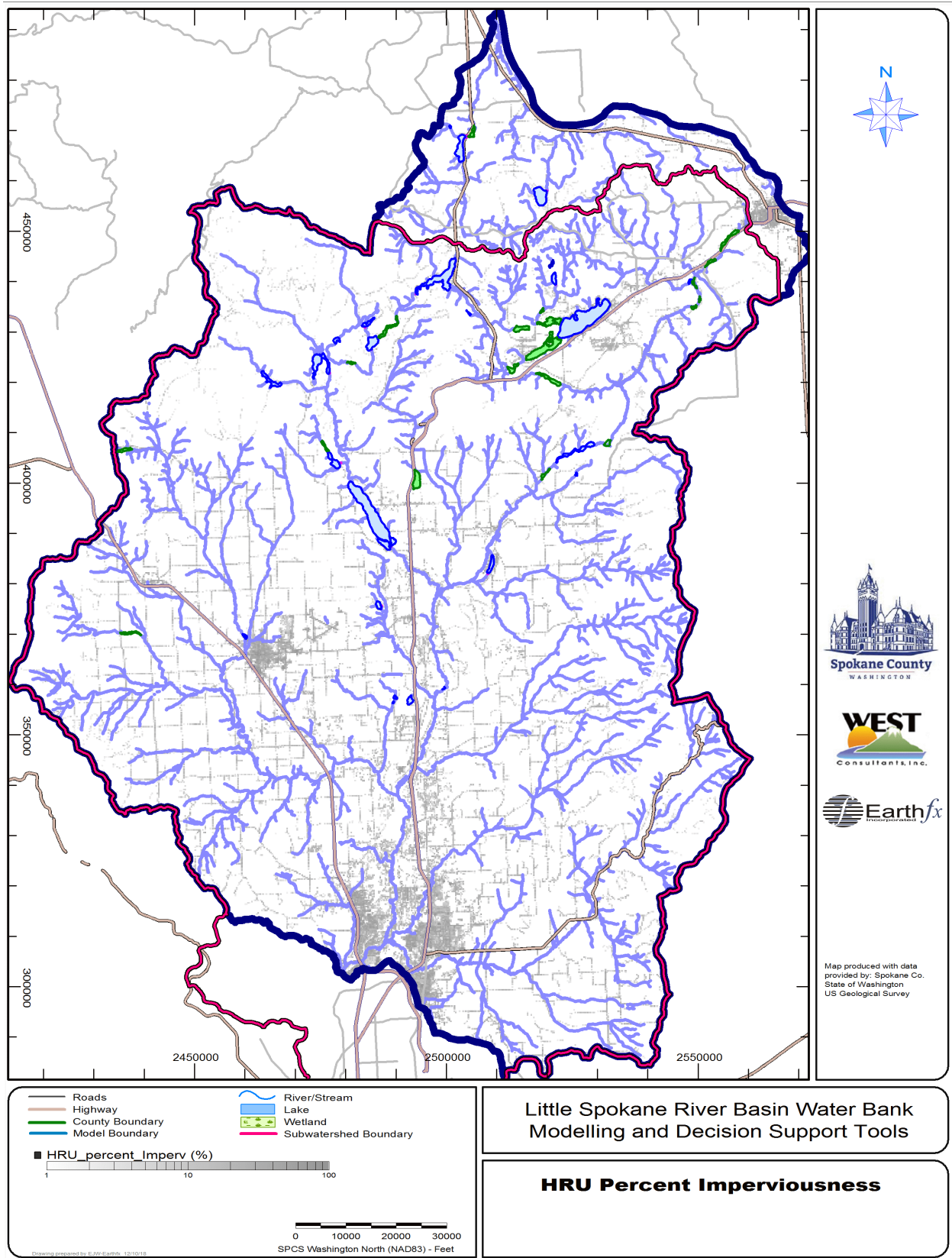
Figure 7.18: Distribution of percent imperviousness (from NLCD, 2011).
