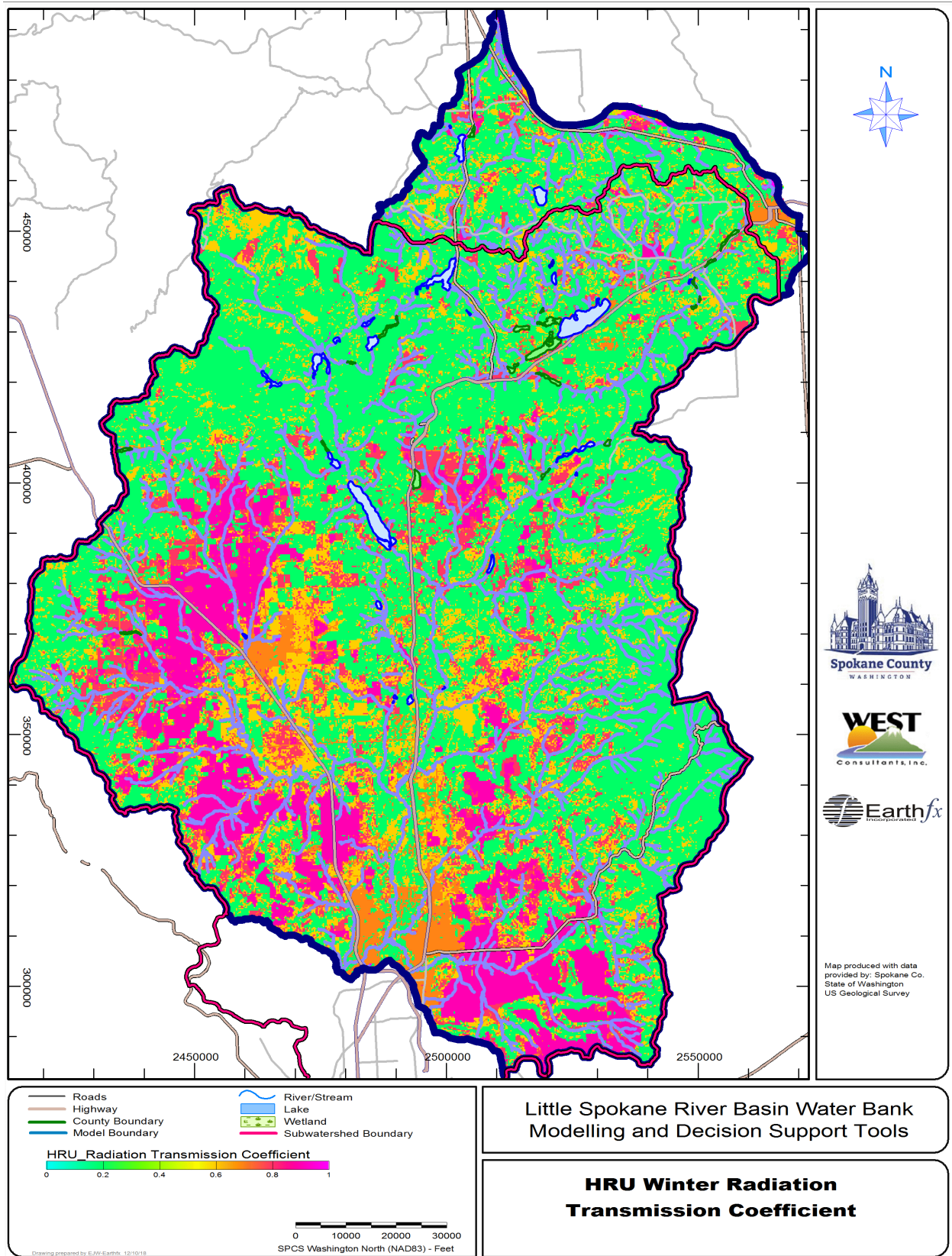
Figure 7.16: Distribution of winter radiation transmission coefficient.
