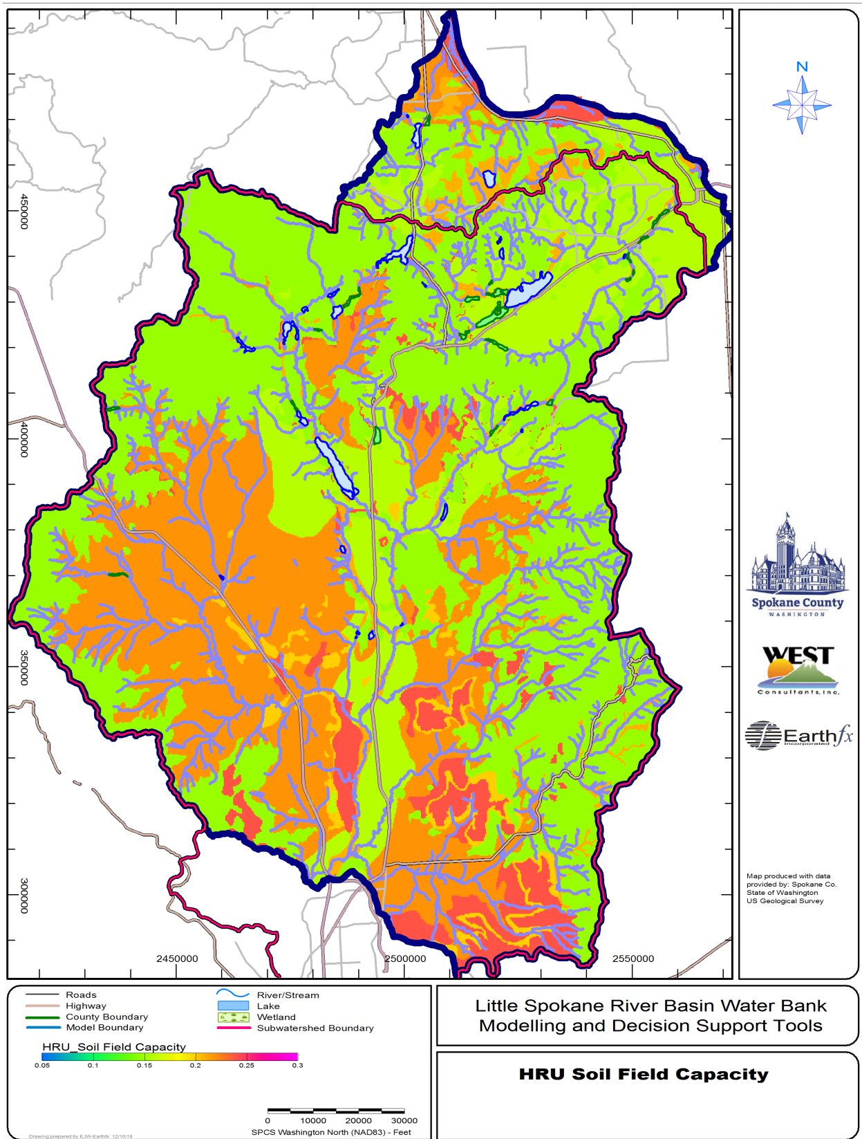
Figure 7.20: Distribution of soil zone field capacity.
