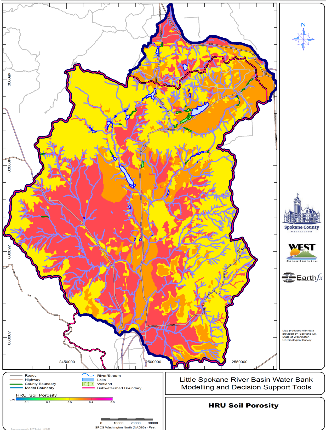
Figure 7.19: Distribution of soil zone porosity.
