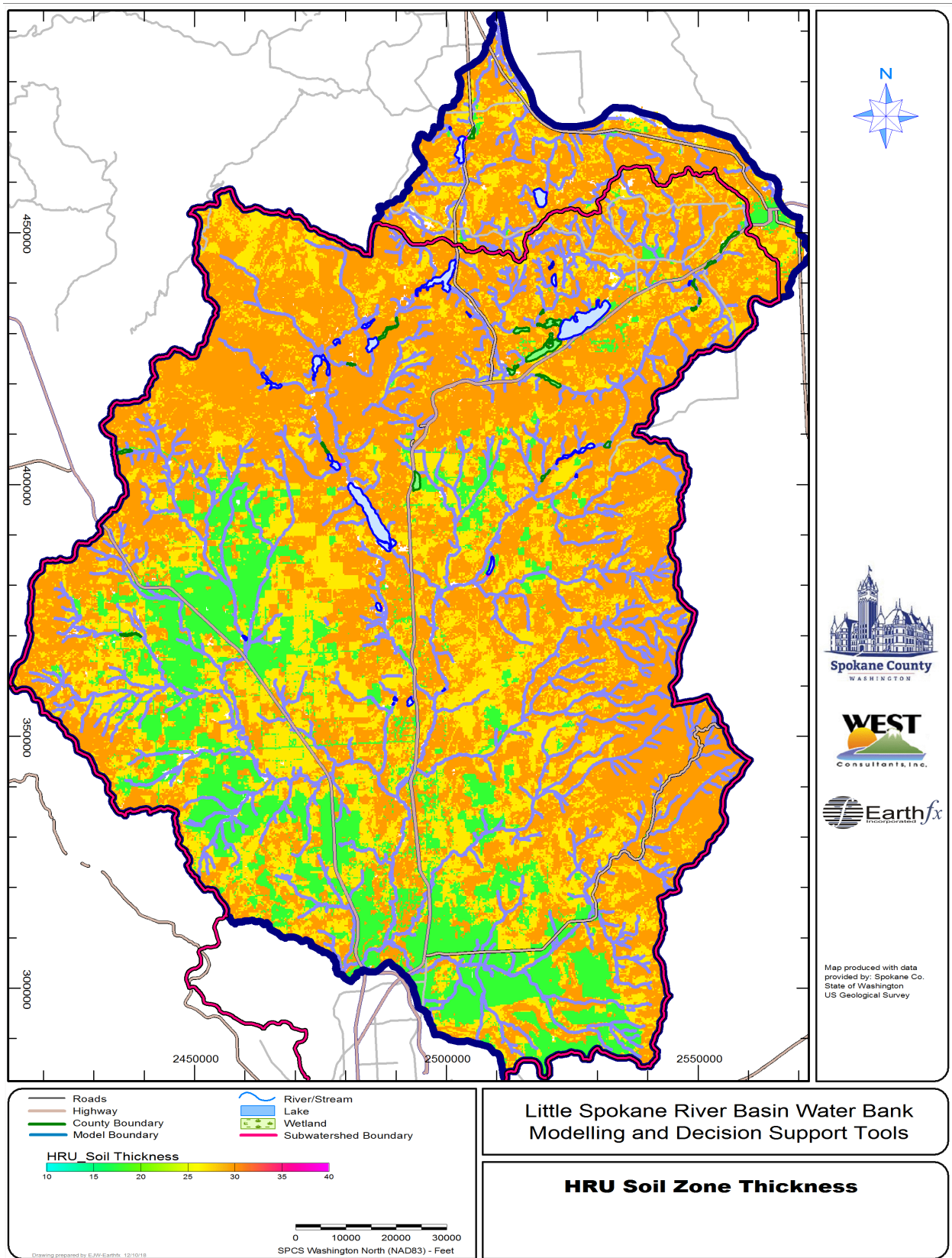
Figure 7.17: Distribution of soil zone thickness (in inches).
