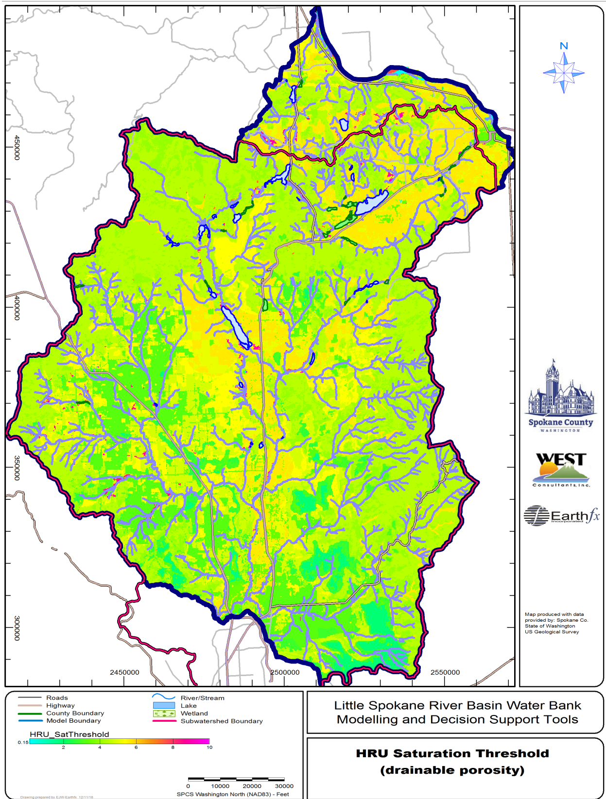
Figure 7.23: Saturation threshold (drainable porosity).
