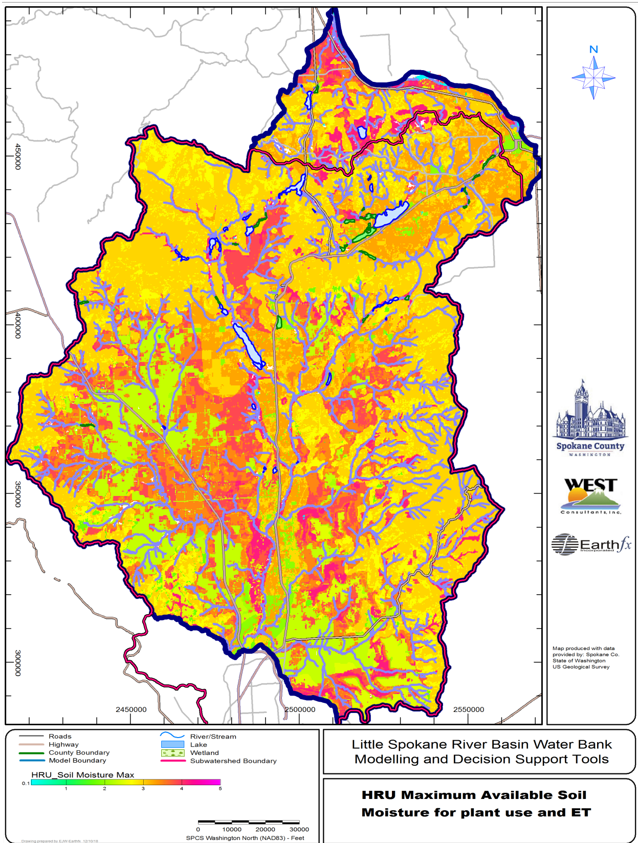
Figure 7.22: Distribution of maximum available soil moisture for ET and plant use.
