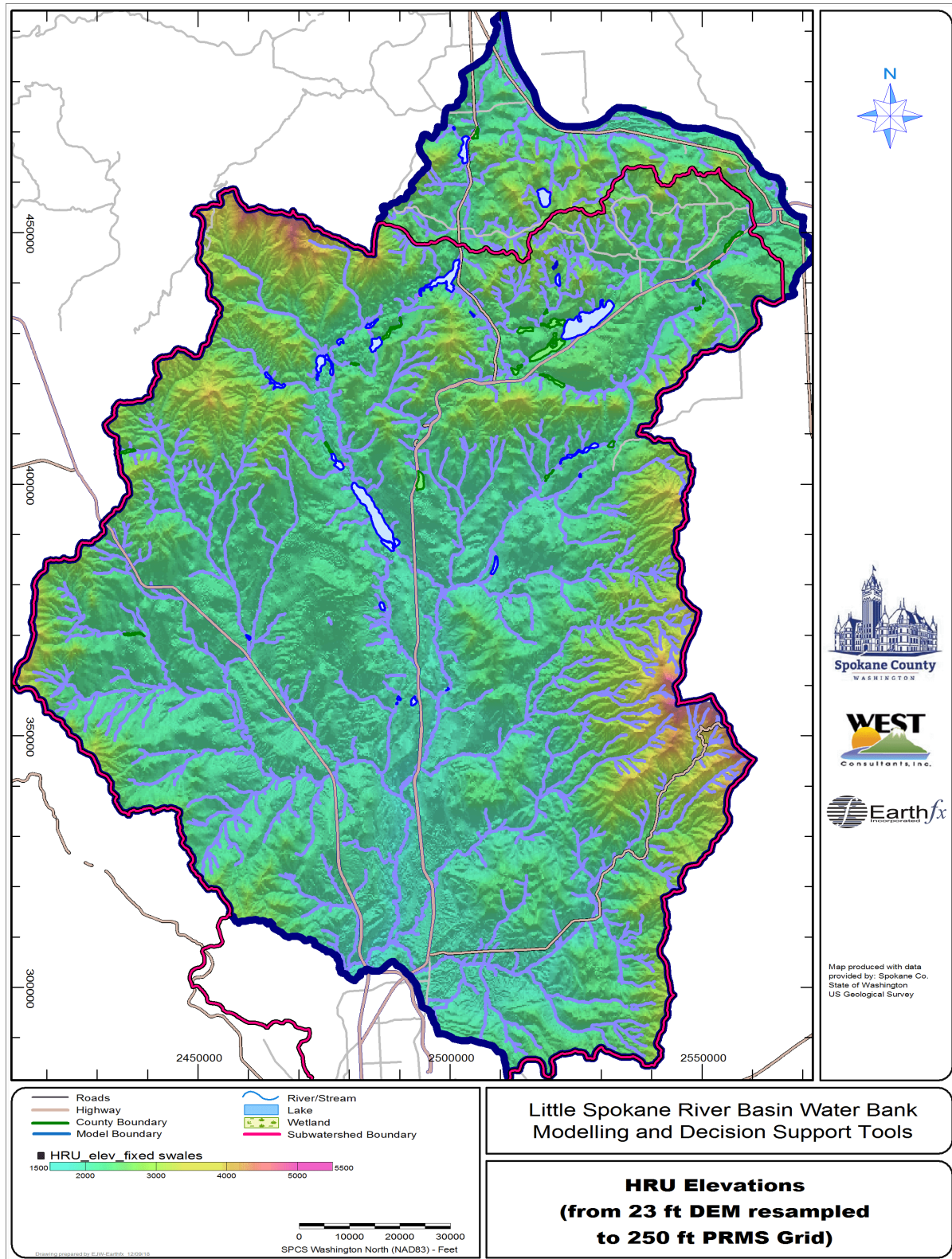
Figure 7.7: HRU elevations (from USGS 23 ft DEM resampled to PRMS grid).
