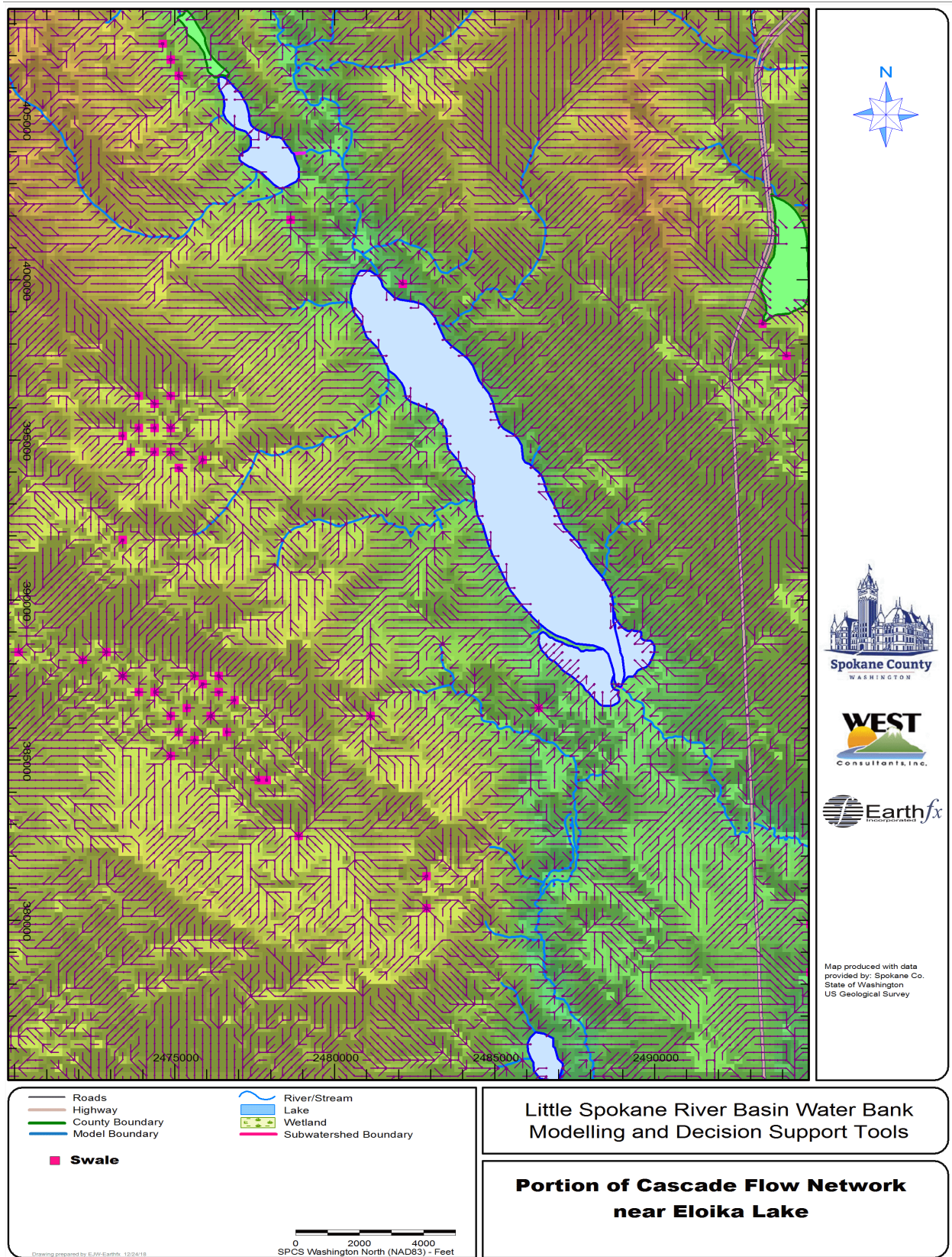
Figure 7.10: Topography and resulting cascade flow network near Eloika Lake
