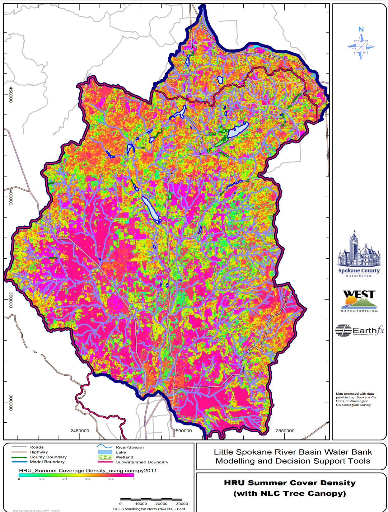
Figure 7.11: Distribution of summer vegetation cover density.
