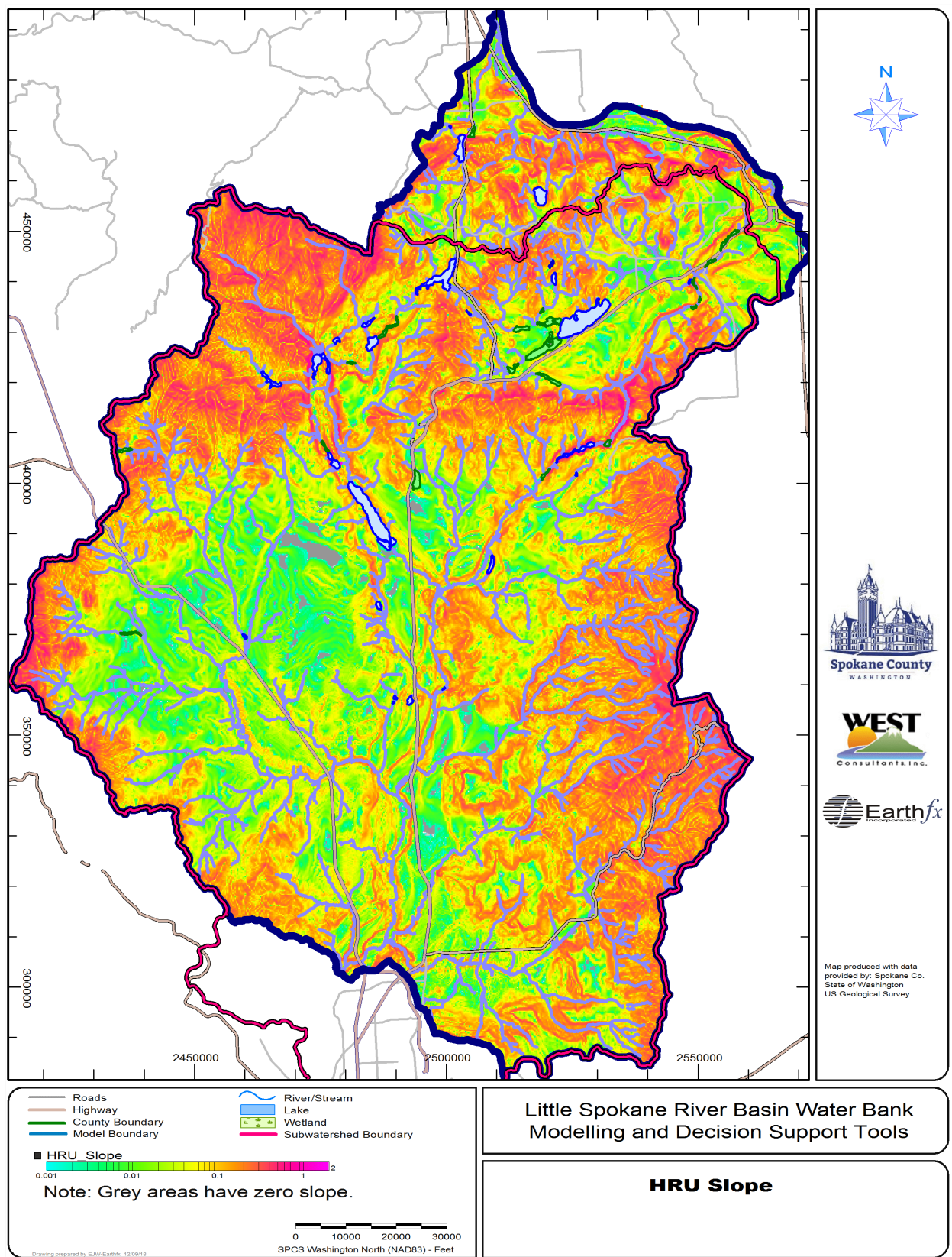
Figure 7.8: Distribution of slope (in ft/ft). Large grey areas with zero slope are artifacts of original DEM.
