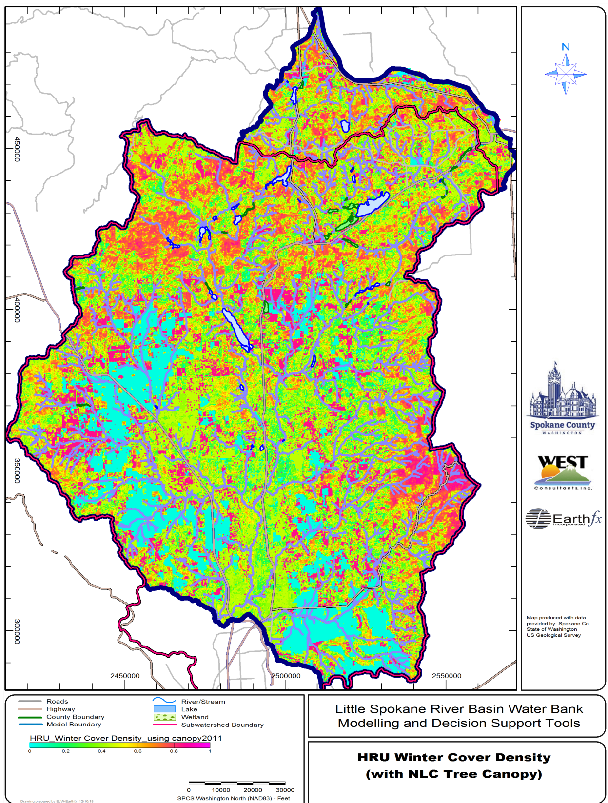
Figure 7.12: Distribution of winter vegetation cover density.
