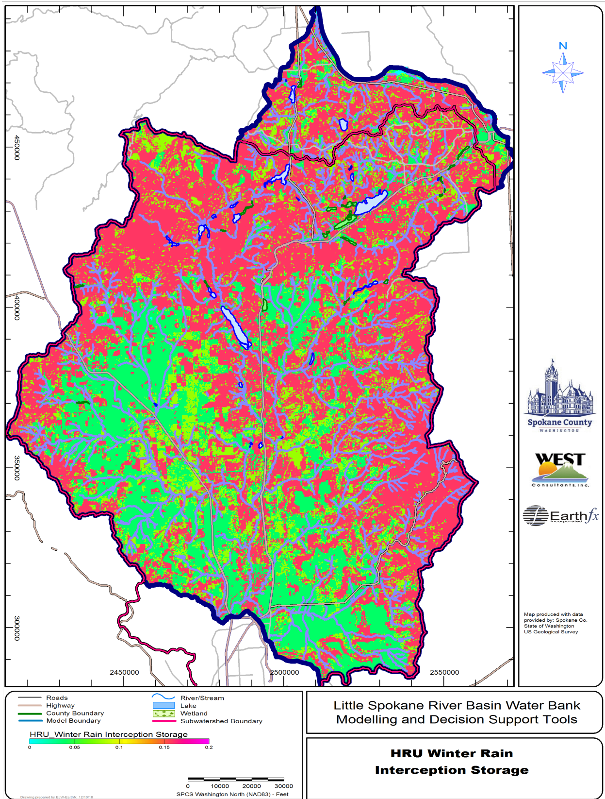
Figure 7.14: Distribution of winter rain interception storage.
