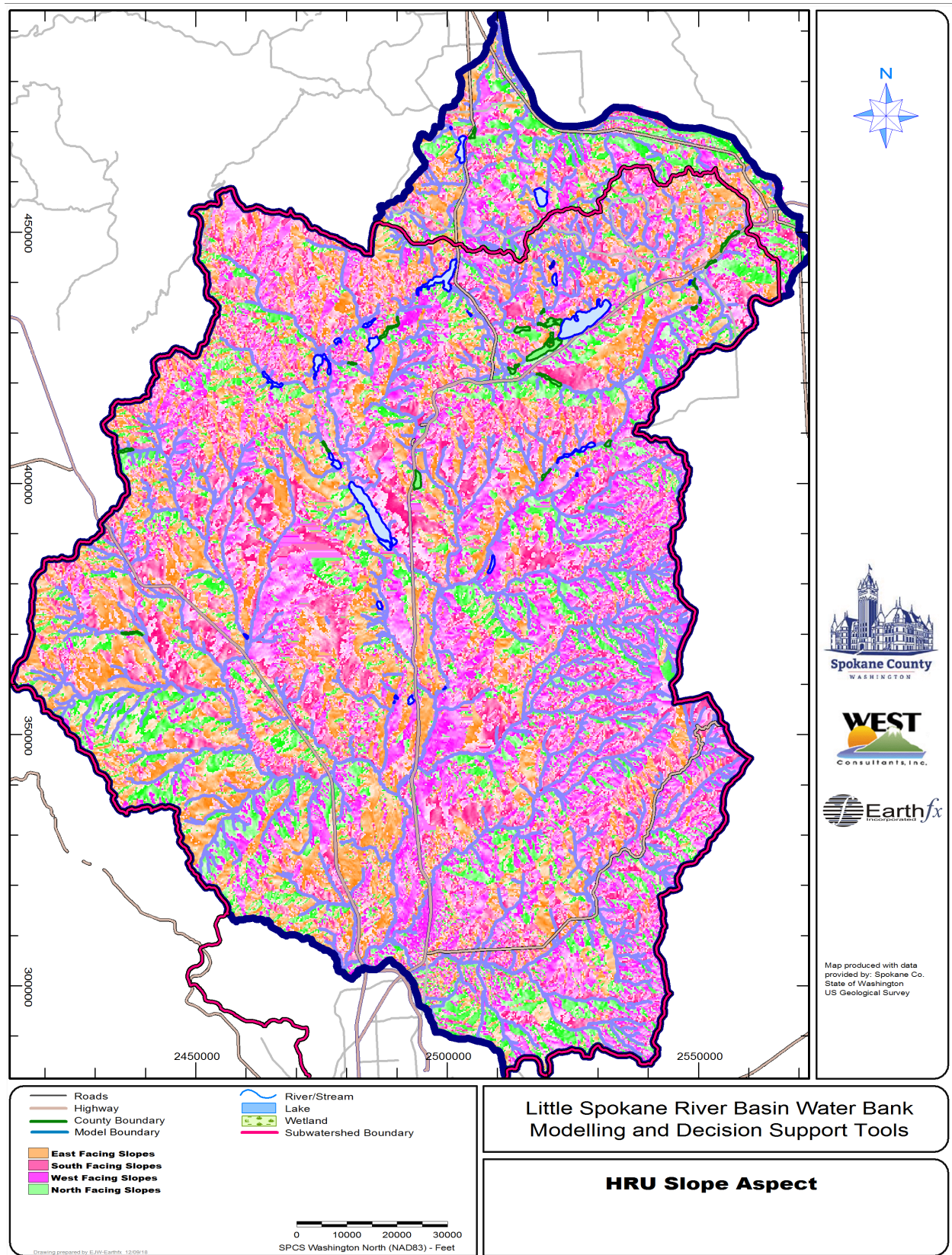
Figure 7.9: Distribution of slope aspect (value of 0 or 360 indicates cell is facing due north).
