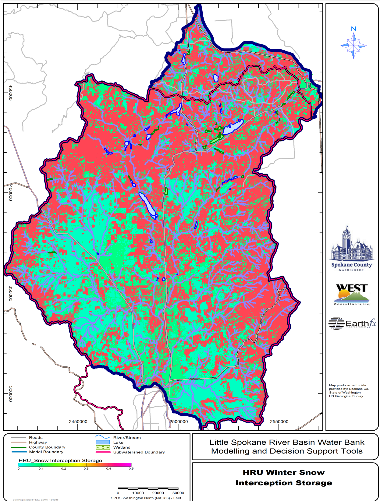
Figure 7.15: Distribution of winter snow interception storage.
