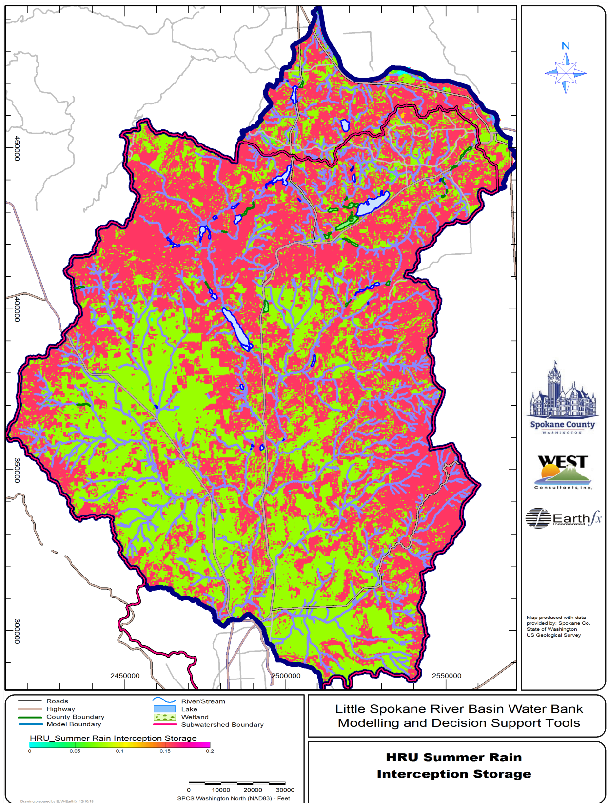
Figure 7.13: Distribution of summer rain interception storage.
