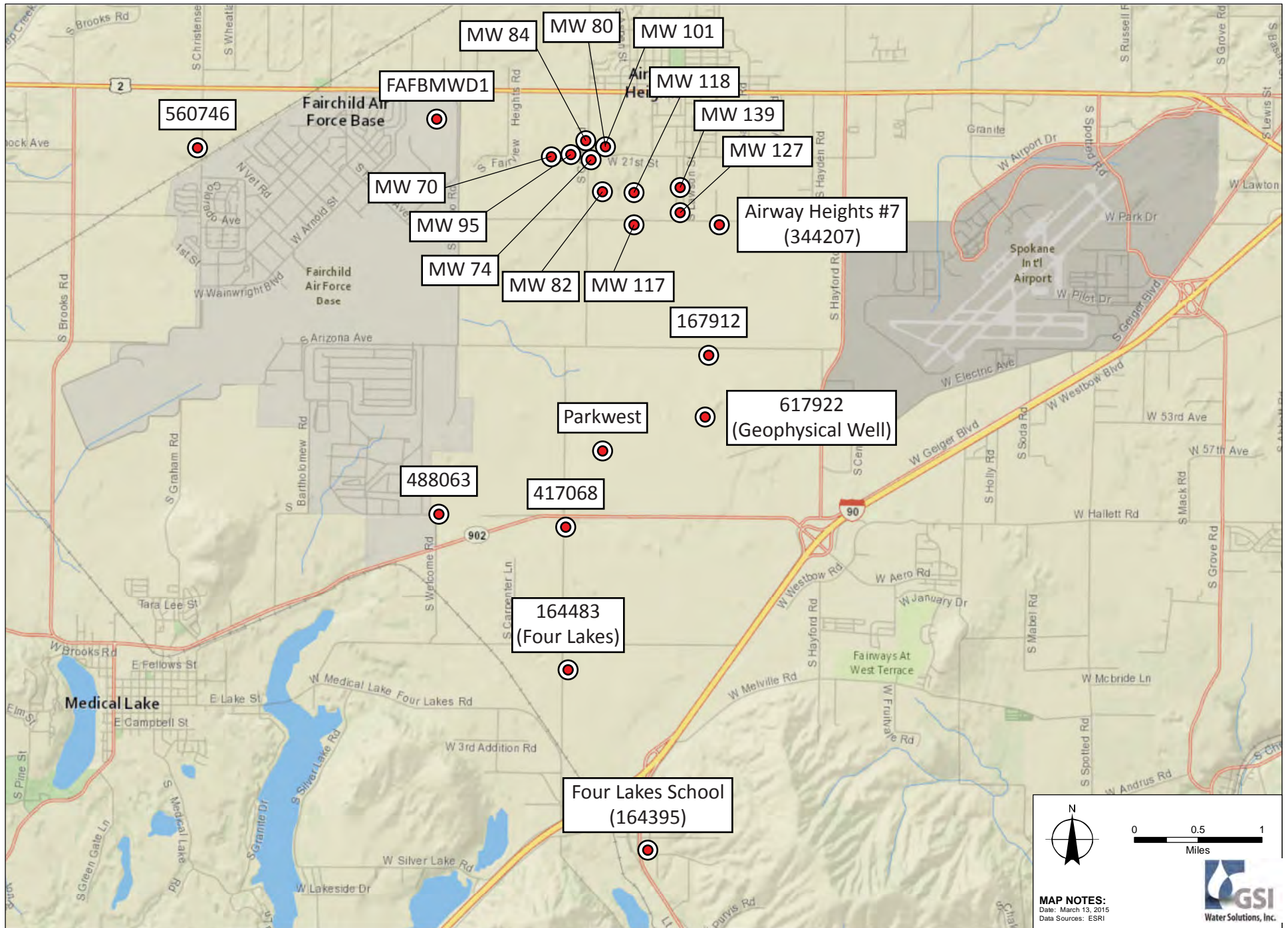
Figure 25. Locations of selected wells in the Central Plains and Craig Road Landfill areas.
