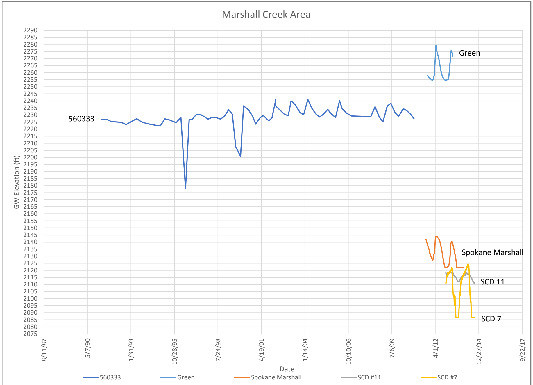
Figure 24. Hydrographs of selected wells in the Marshall Creek area.
