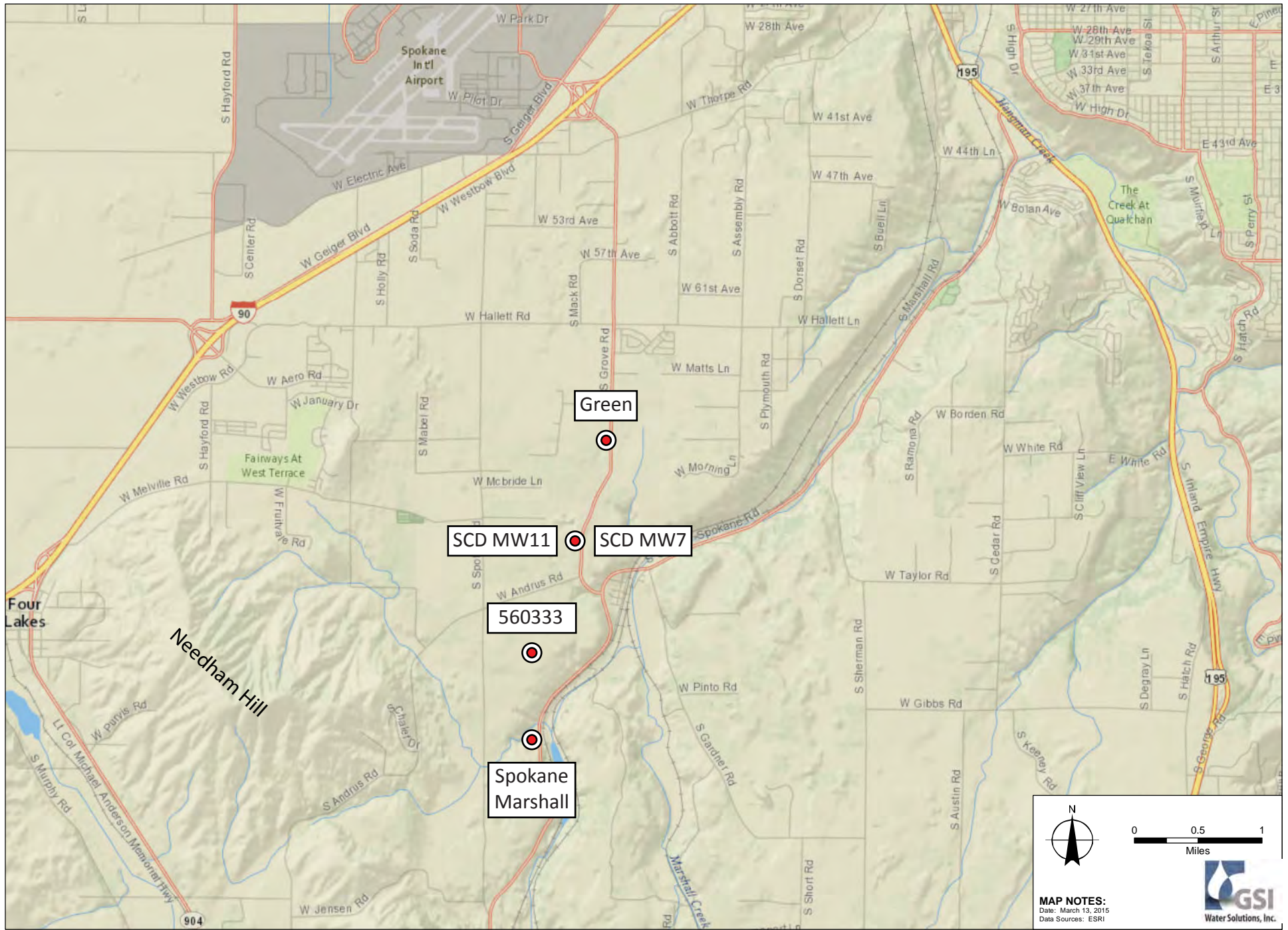
Figure 23. Locations of selected wells in the Marshall Creek area.
