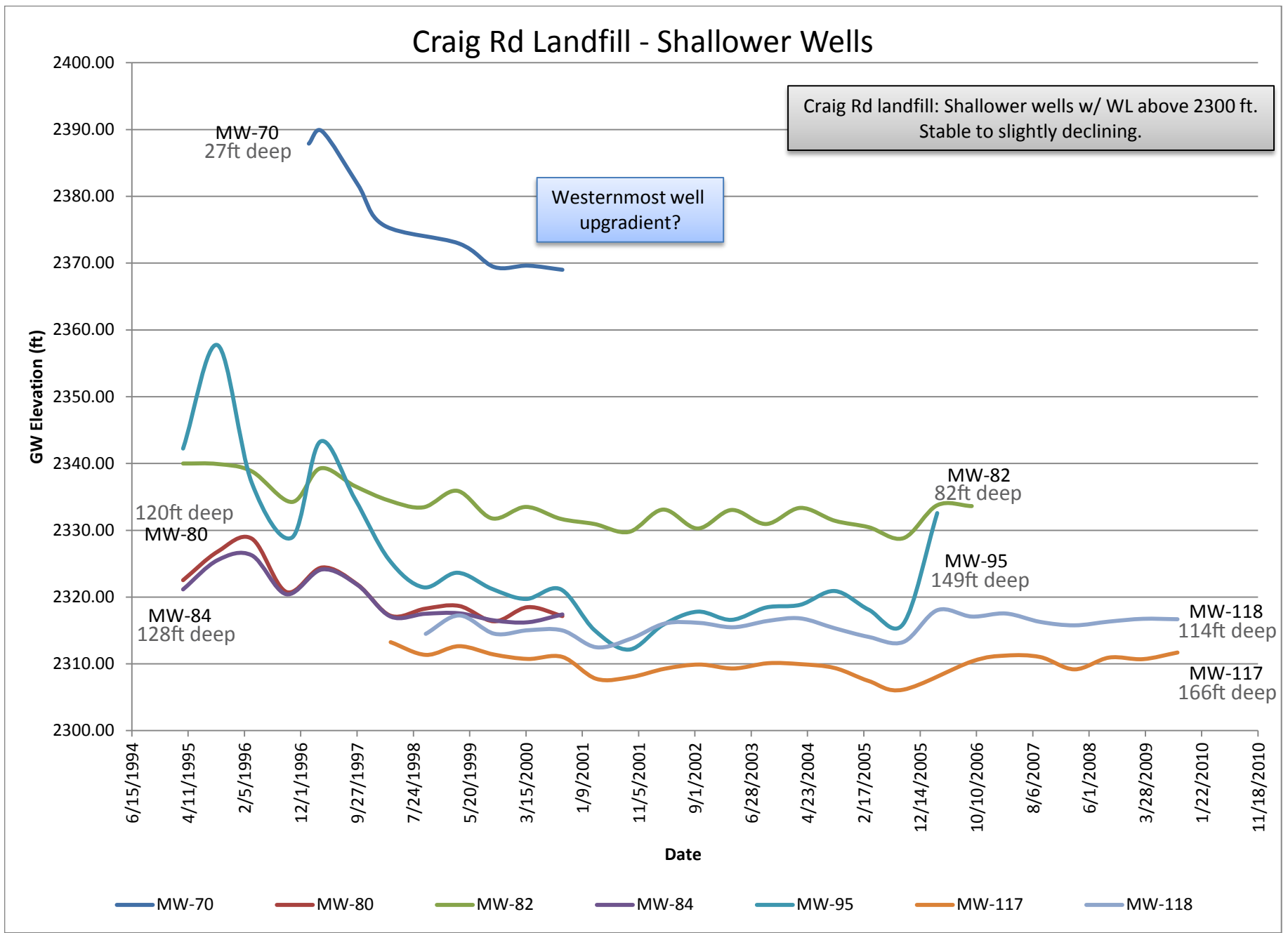
Figure 27. Hydrographs of selected shallower wells in the Craig Road Landfill area.
