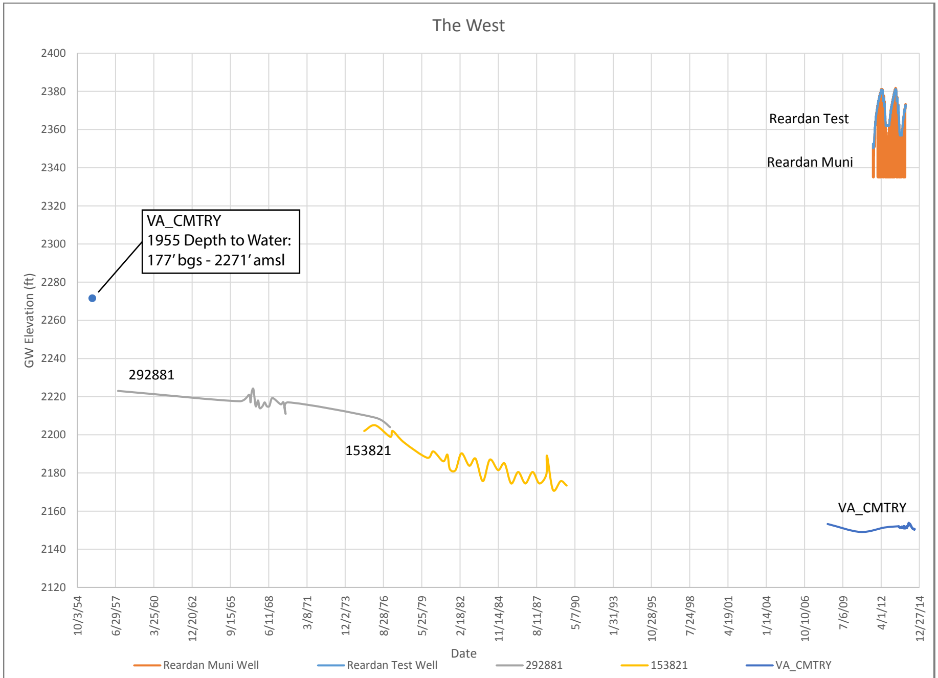
Figure 21. Hydrographs of selected wells in the Western area.
