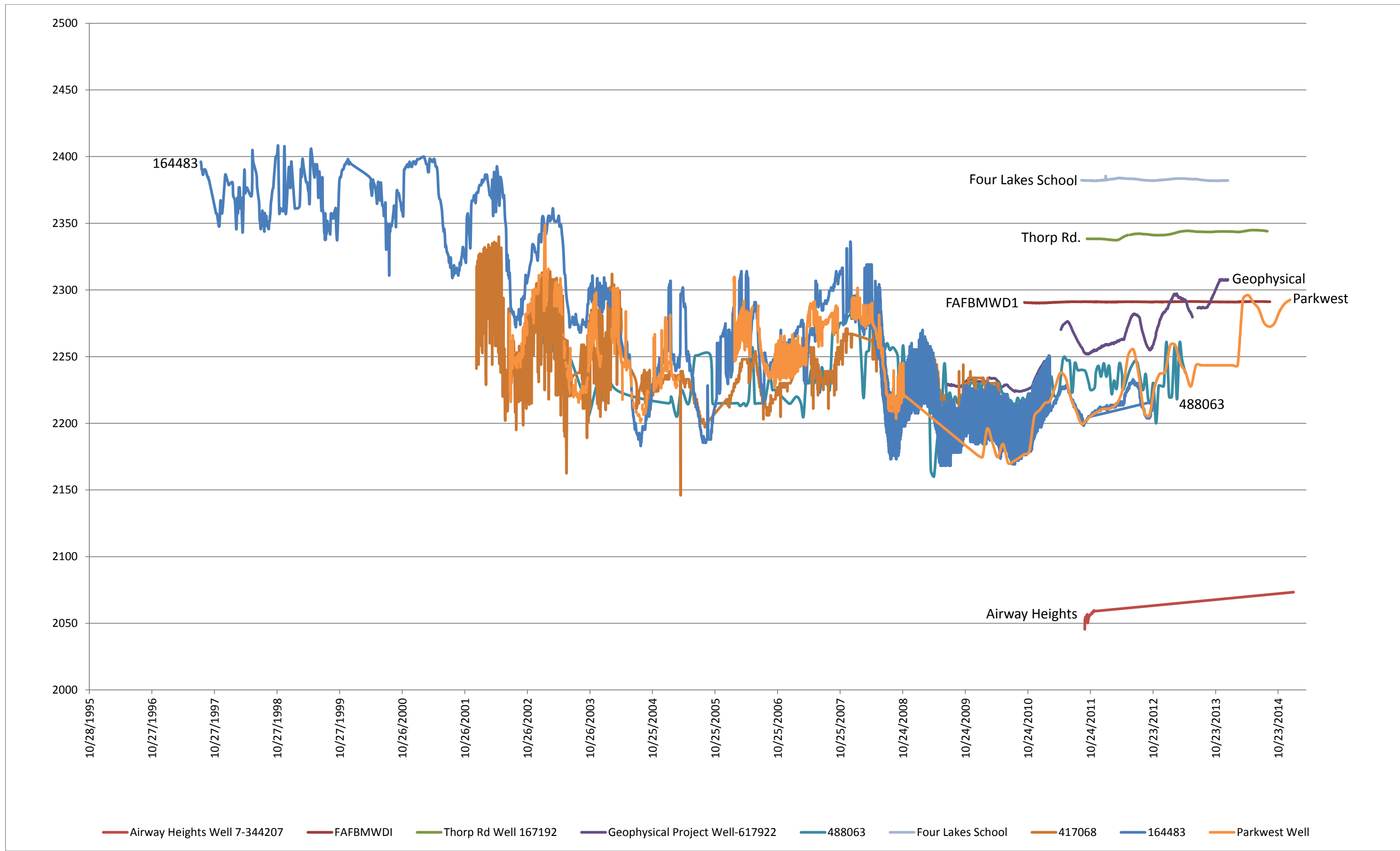
Figure 26. Hydrographs of selected wells in and around the Central West Plains area.
