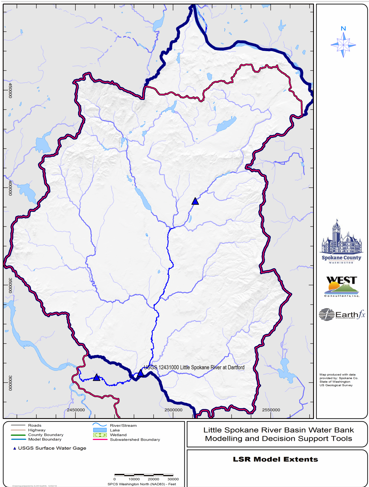
Figure 1.2: Extents of the Little Spokane River (LSR) Model area.
