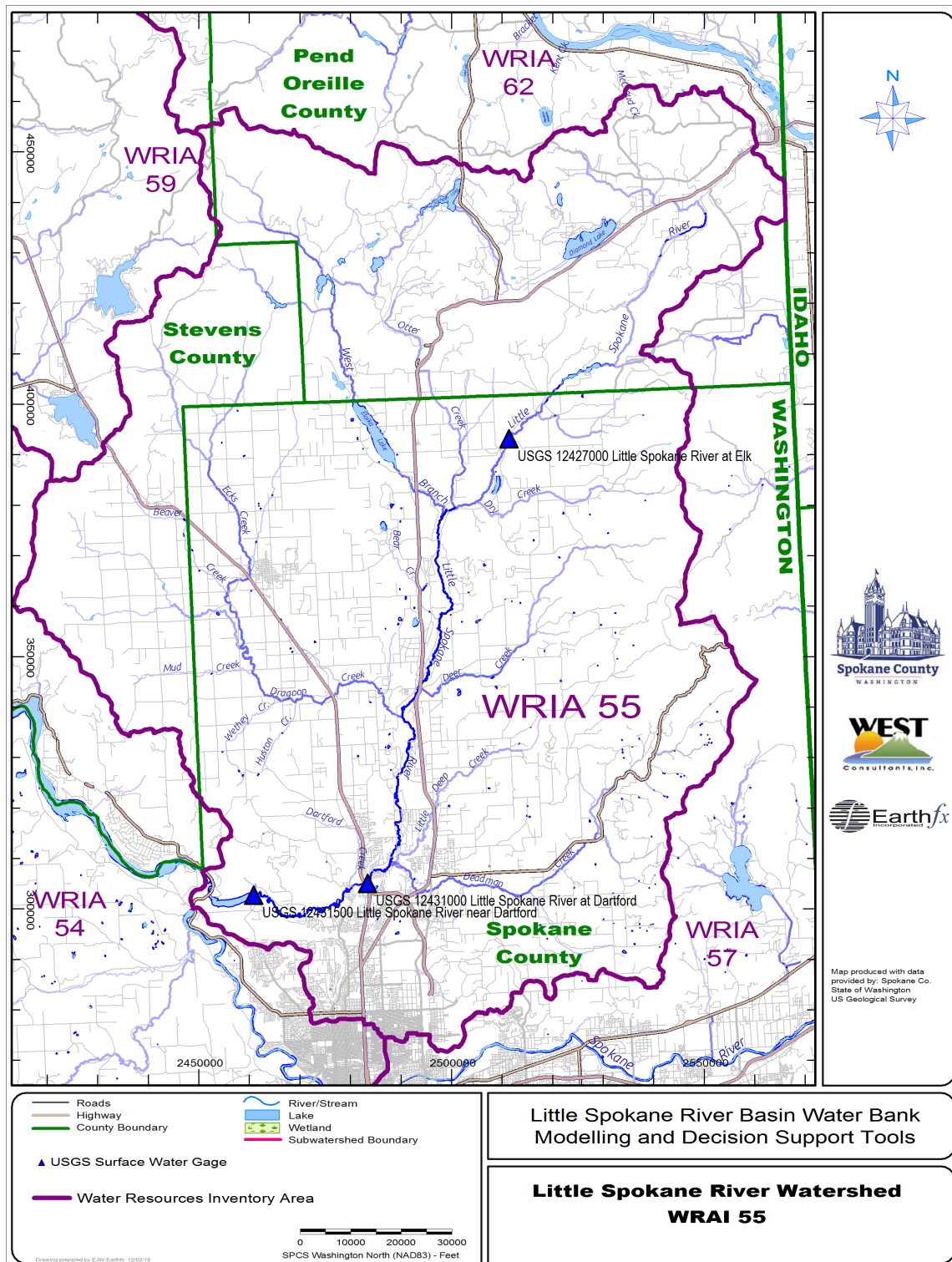
Figure 1.1: Little Spokane River watershed - Water Resource Inventory Area - WRIA 55.
